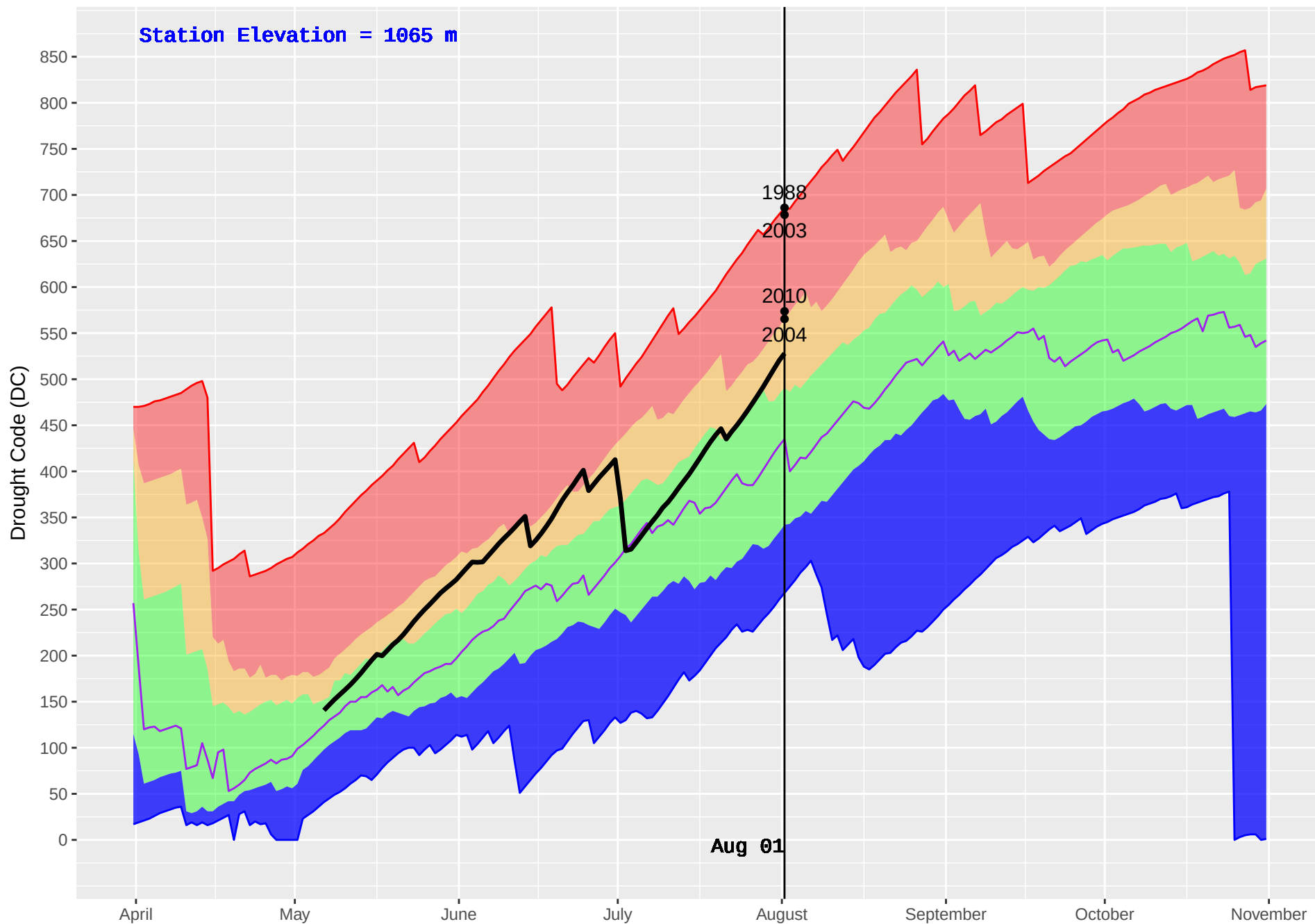
PLACE LAKE (212) : Historical (1981–2016) and Current (2018) Daily Drought Code (DC)
